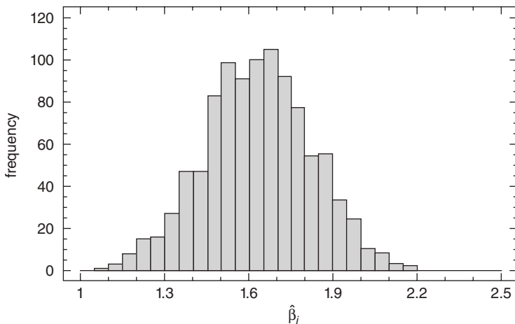
Figure 15.8 Histogram of bootstrap \hat{\beta}_1^* , Example 15.3.
