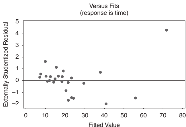
Figure 4.6 Plot of externally studentized residuals versus predicted for the delivery time data.
