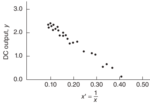
Figure 5.7 Plot of DC output versus x' = 1/x for the windmill data.
