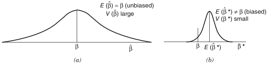
Figure 9.4 Sampling distribution of (a) unbiased and (b) biased estimators of \beta . (Adapted from Marquardt and Snee [1975], with permission of the publisher.)
