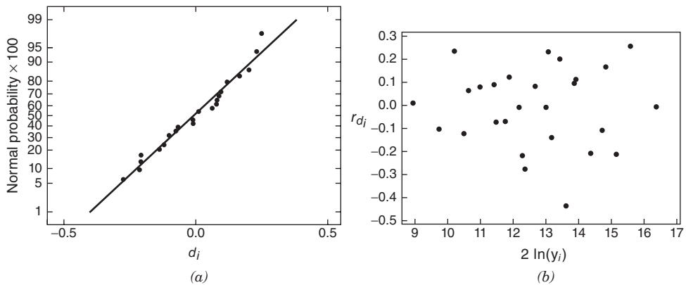
Figure 13.7 Plots of the deviance residuals from the GLM for the worsted yarn data. (a) Normal probability plot of deviance results. (b) Plot of the deviance residuals versus 2\ln(\hat{y}_i)
