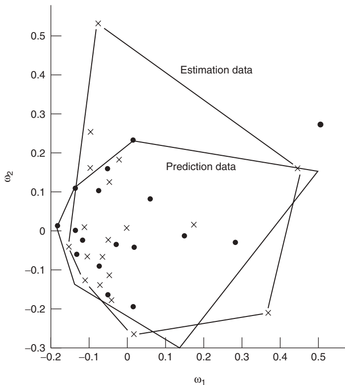
Figure 11.2 Estimation data (x) and prediction data (•) using orthonormalized regressors.
