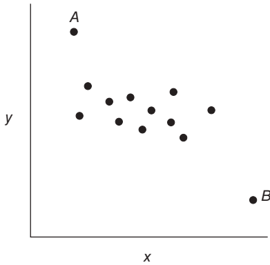
Figure 2.8 Two influential observations.
